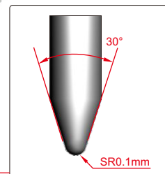
sharp point indenter
