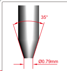
blunt taper indenter
